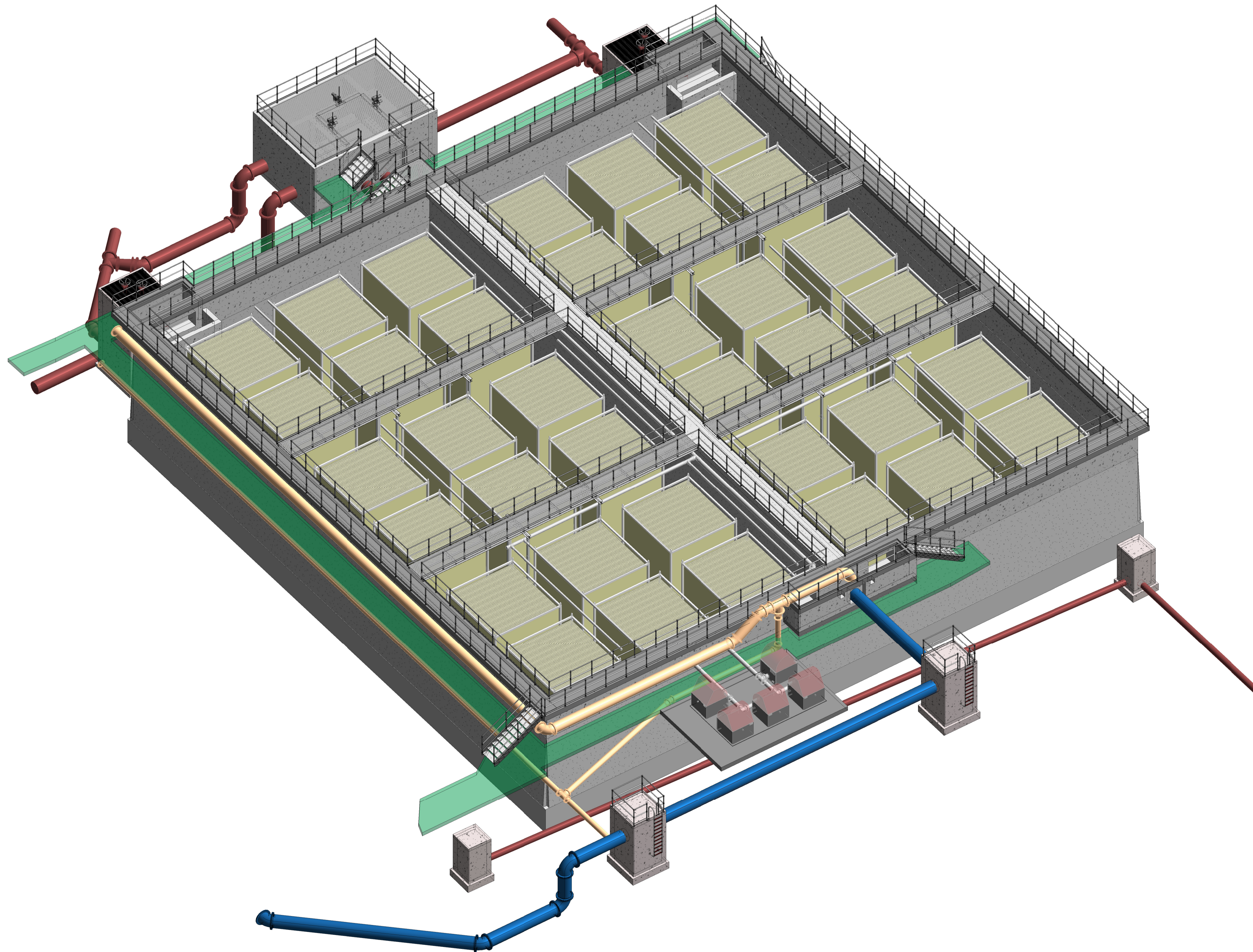
1 3D VIEW OF AF AERATION TANK
